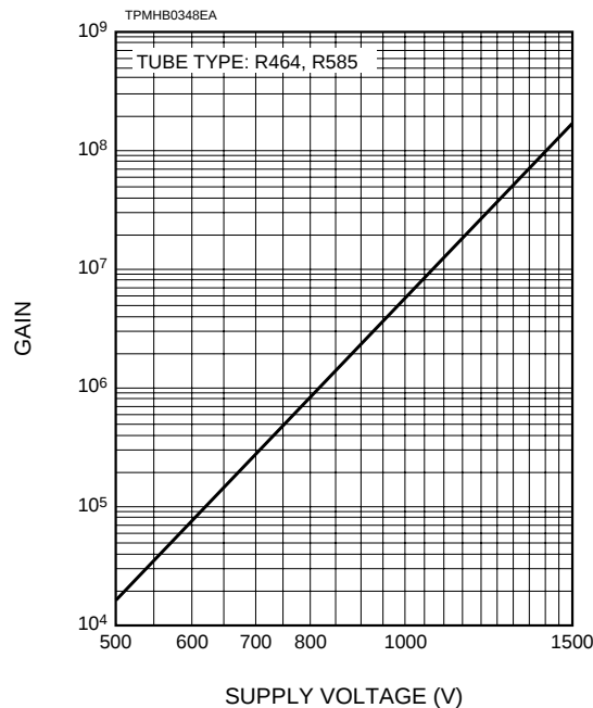
Figure 2: Typical Gain
