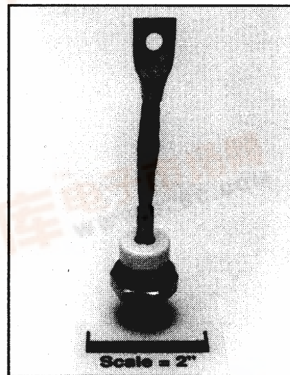
R502_13/R503_13 Fast Recovery Rectifier 125 Amperes Average, 1400 Volts
