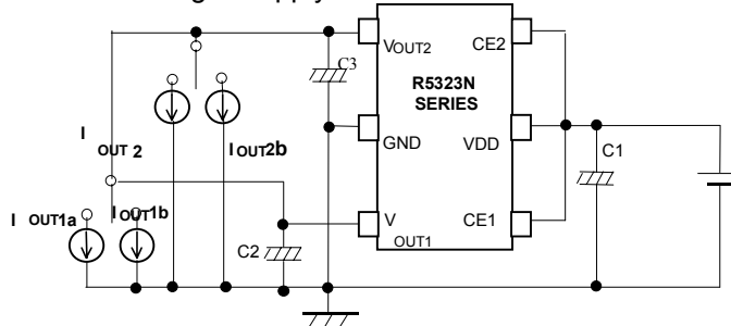
Fig.2 Supply Current Test Circuit
