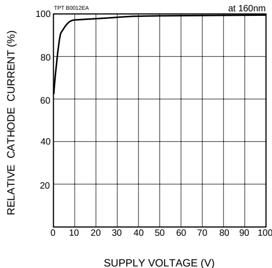
Figure 2: Saturation Characteristics
