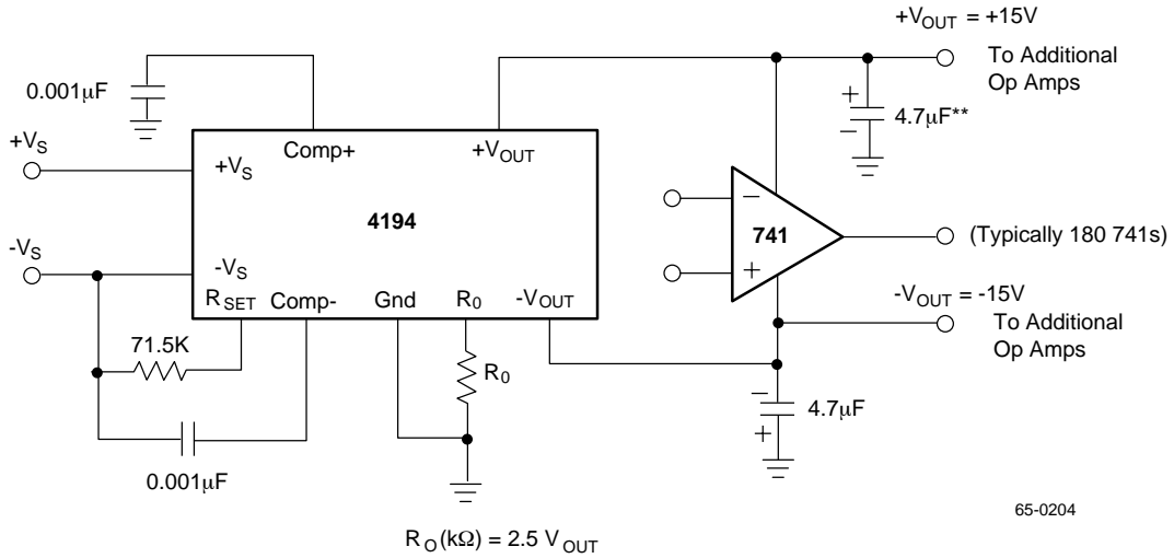
Figure 6. Balanced Output Voltage — Op Amp Application
