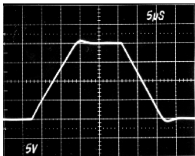
STEP RESPONSE NO LOAD
