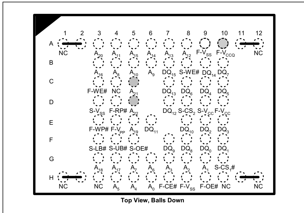
Figure 1. 66-Ball SCSP
