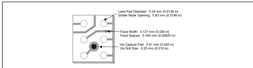
Figure 14. Standard PCB Design Rules Can be Used with SCSP Device
