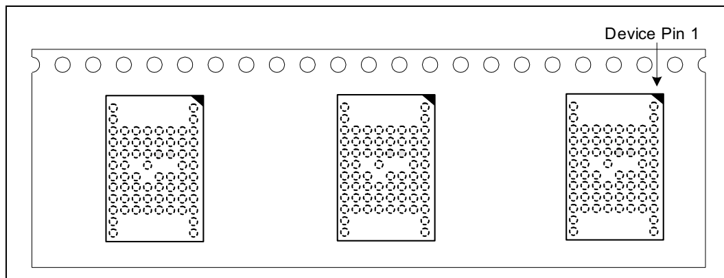
Figure 23. SCSP Device in 24 mm Tape (10 mm x 8 mm and 12 mm x 8 mm)
