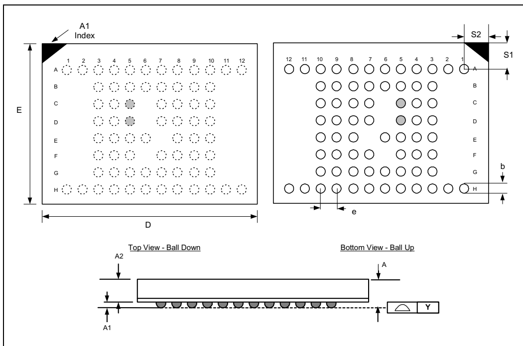
Figure 21. SCSP: 12 x 8 Ball Matrix
