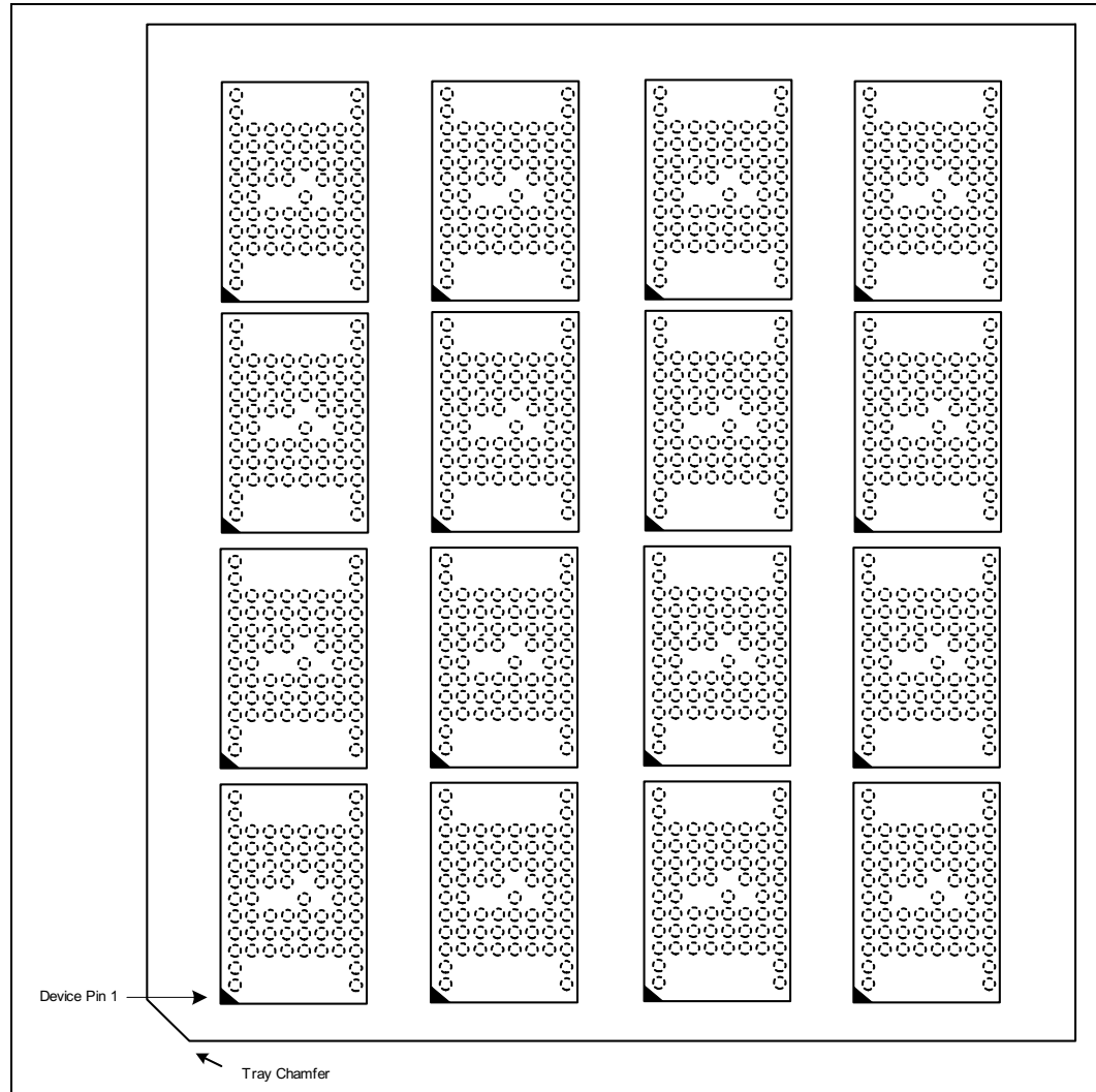
Figure 22. SCSP Device in Tray Orientation (10 mm x 8 mm and 12 mm x 8 mm)
