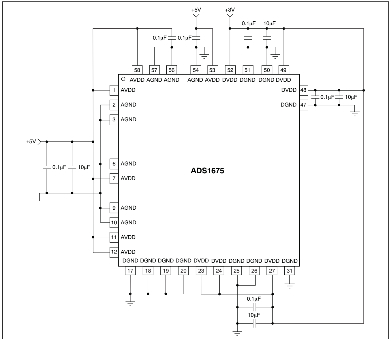
Figure 52. Power-Supply Decoupling
