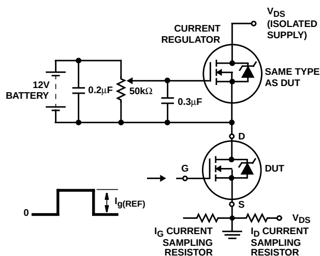
FIGURE 20. GATE CHARGE TEST CIRCUIT
