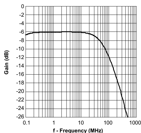
Figure 83. Low-Pass Filter Measured Frequency Response
