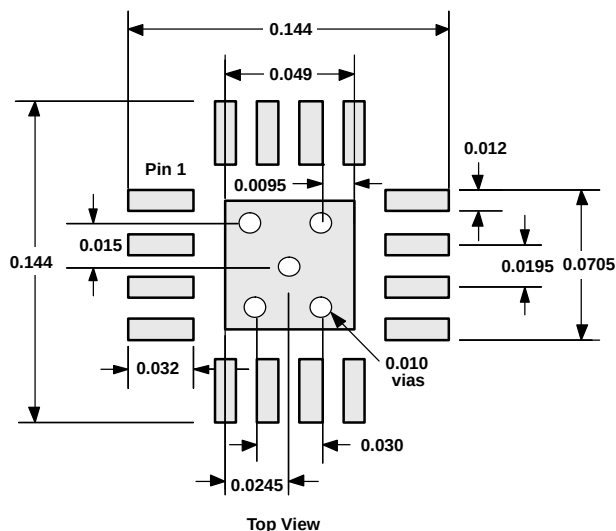
Figure 87. QFN Etch and Via Pattern
