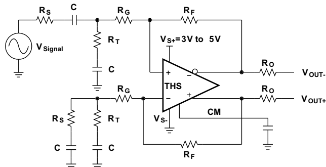
Figure 81. THS4513 AC Coupled Single-Supply
