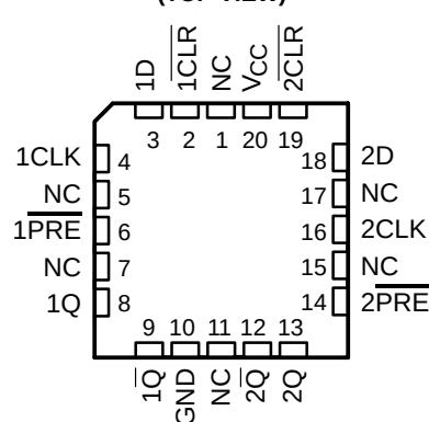
SN54AHCT74 ... FK PACKAGE (TOP VIEW)
