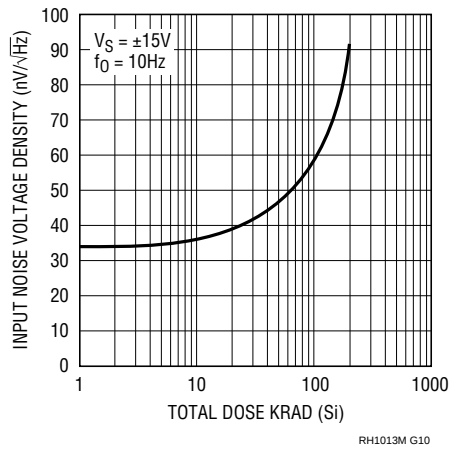
Input Noise Voltage Density
