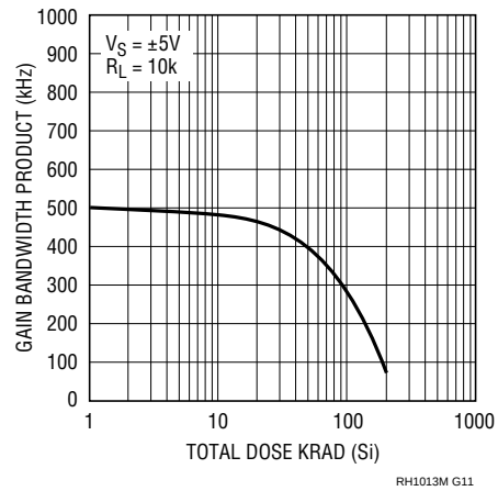
Gain Bandwidth Product
