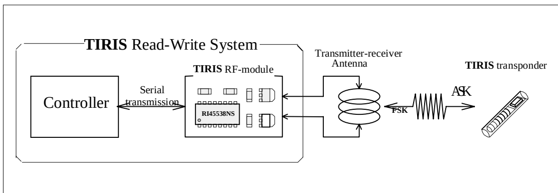
TIRIS System Configuration
