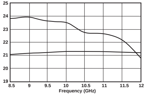
RMWB12001 12 GHz BA, Power Output and Gain at 3 dB Compression Vs. Frequency and Temperature On-Wafer Measurements, V_d=4 V, I_{dq}=96 mA, T=25^\circ\text{C}
