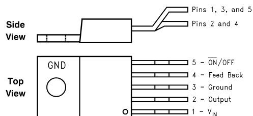
Bent and Staggered Leads, Through Hole Package 5-Lead TO-220 (T)
