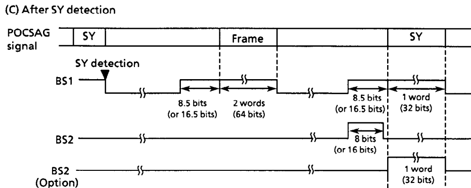
Figure 19 Battery saving
