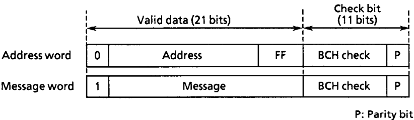
Figure 21 Address and message word configuration
