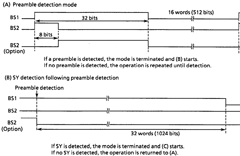
Figure 19-1 Battery saving
