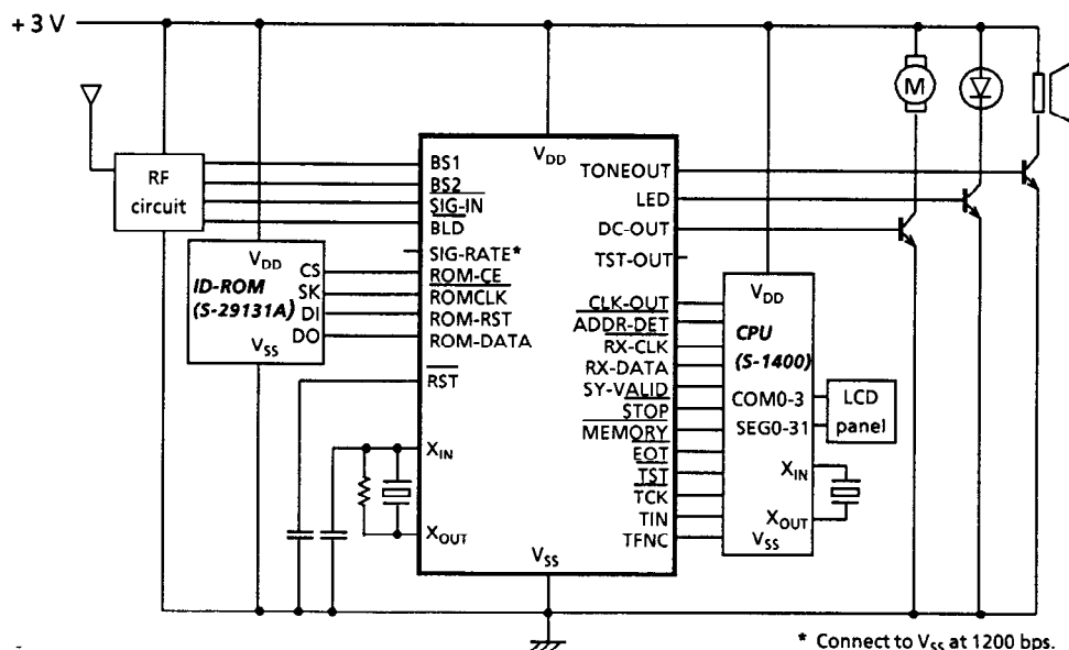
Figure 34 Application circuit example: Display pager
