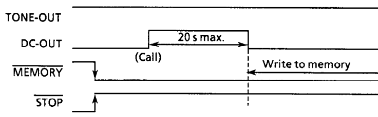
Figure 22 Memory write timing
