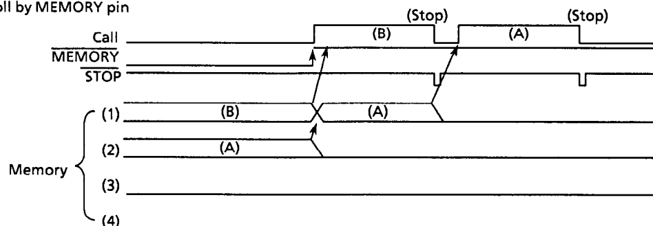
Figure 24 Scroll timing
