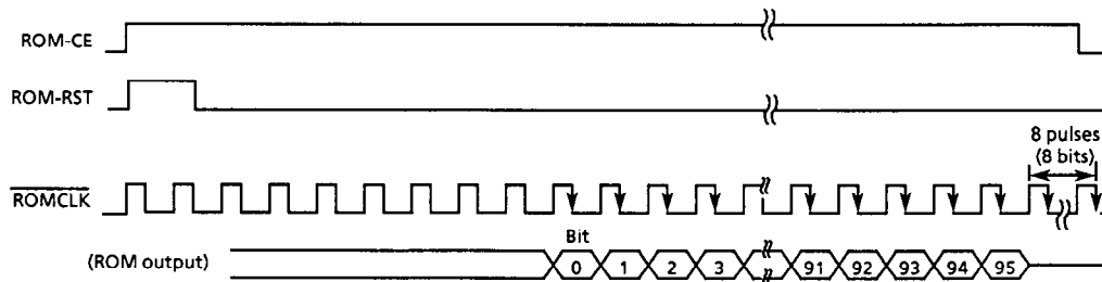
Figure 24 ID-ROM interface
