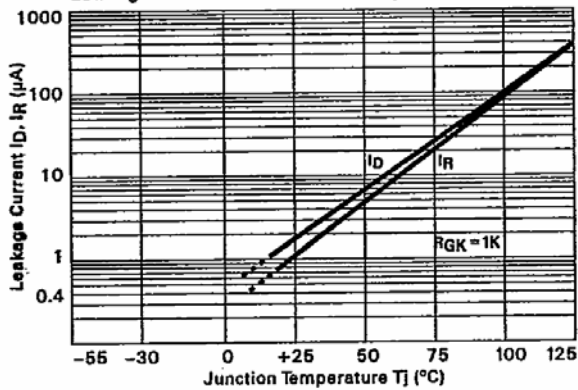
Leakage Current vs Junction Temperature (typical)
