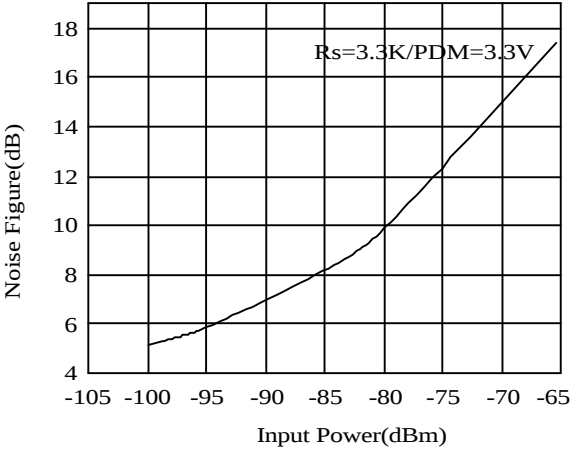
GRPH 2-6 S1M8656A FM Noise Figure
