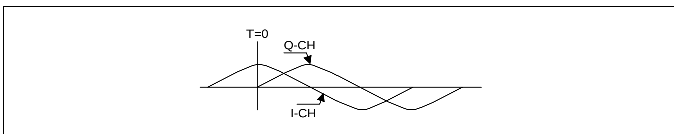
Figure 5. Received I/Q Phase in S1M8656A
