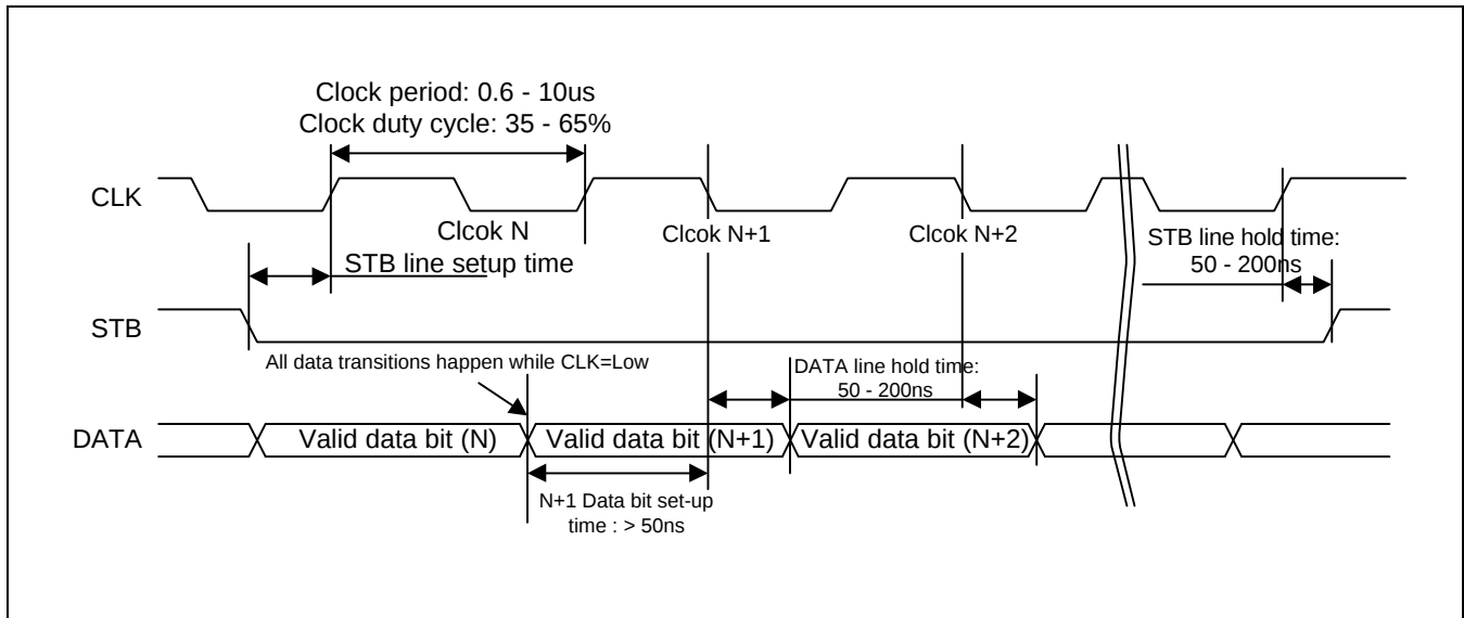
Figure 3. 3-Line Serial Port Interface Timing
