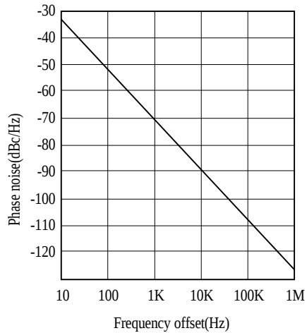
GRPH 2-1 S1M8656A VCO Open Loop Phase Noise at RXVCO_OUT
