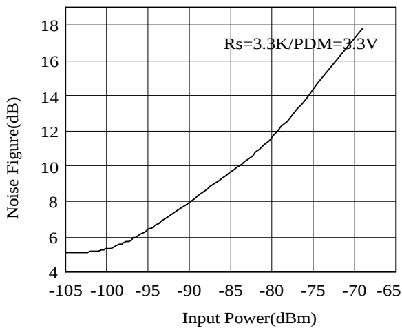
GRPH 2-3 S1M8656A CDMA Noise Figure
