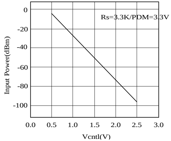
GRPH 2-2 S1M8656A Input Power vs. Vcntl Performance for CDMA full-scale output.
