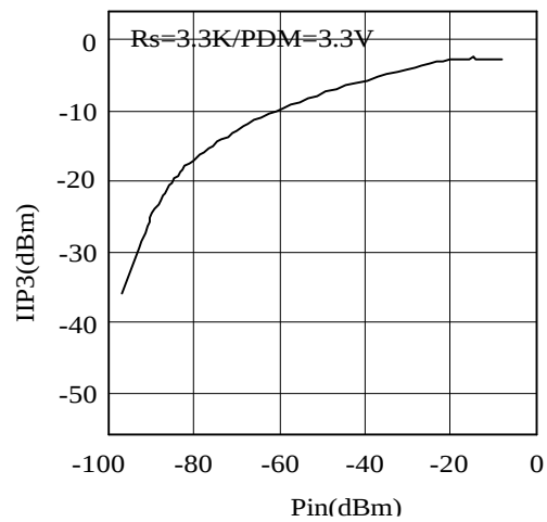
GRPH 2-4 S1M8656A IIP3 for CDMA half-scale output
