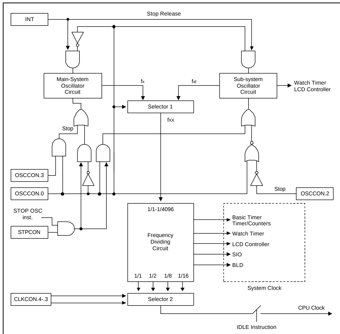
Figure 7-7. System Clock Circuit Diagram
