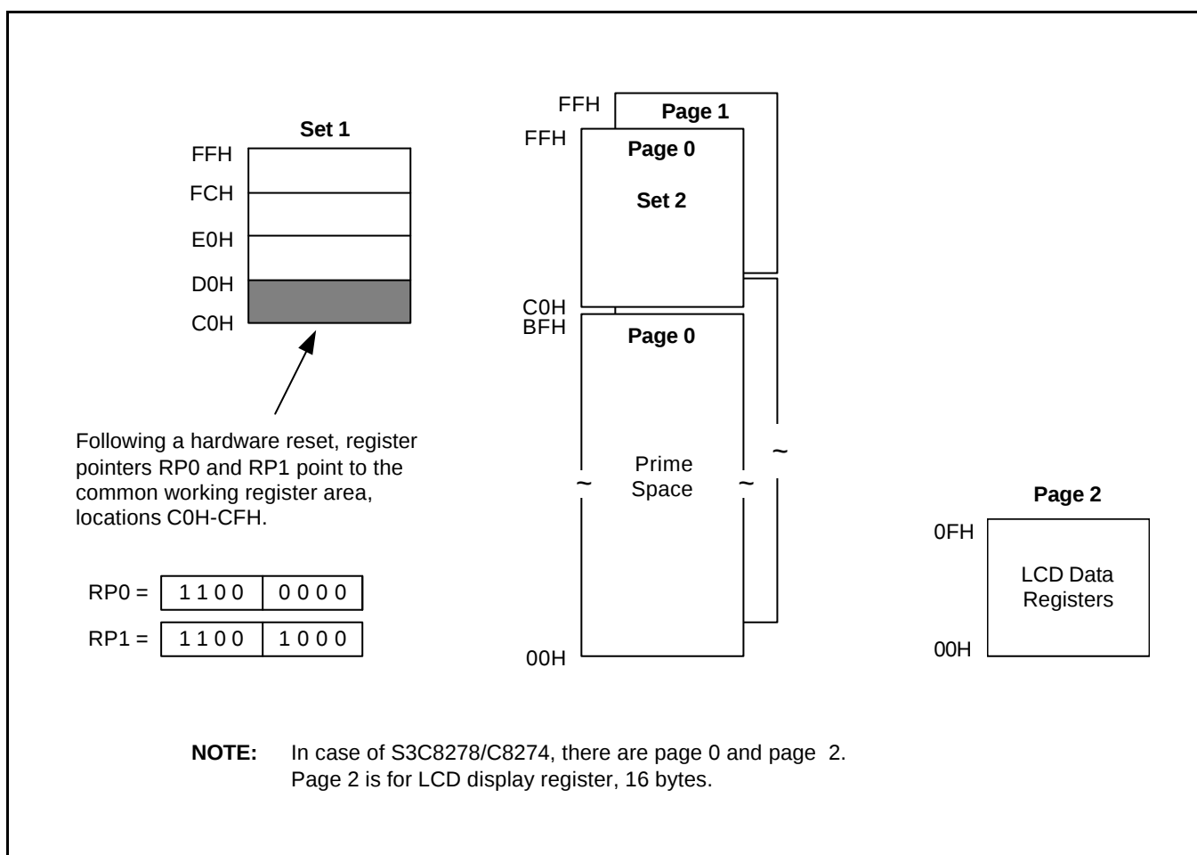
Figure 2-12. Common Working Register Area
