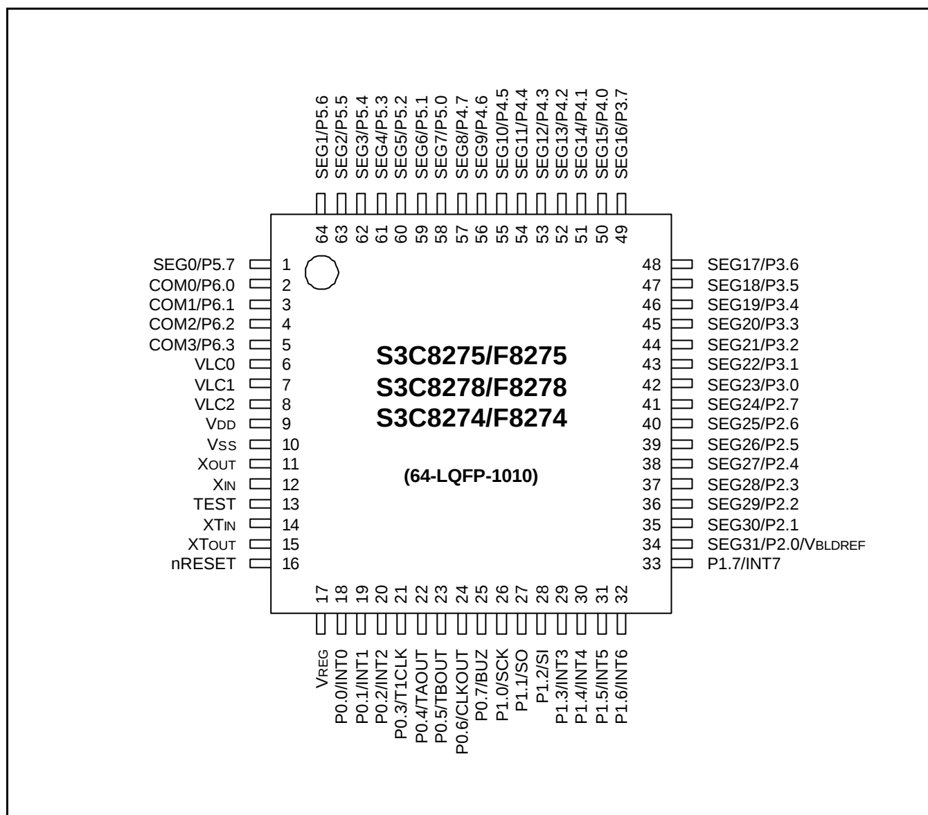
Figure 1-3. S3C8275/F8275/C8278/F8278/C8274/F8274 Pin Assignments (64-LQFP-1010)
