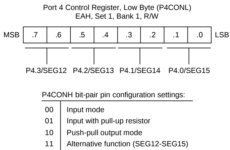
Figure 9-20. Port 4 Low-Byte Control Register (P4CONL)
