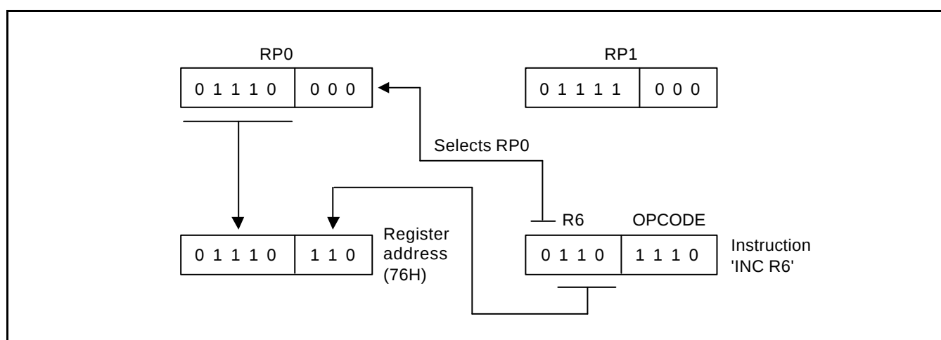
Figure 2-14. 4-Bit Working Register Addressing Example
