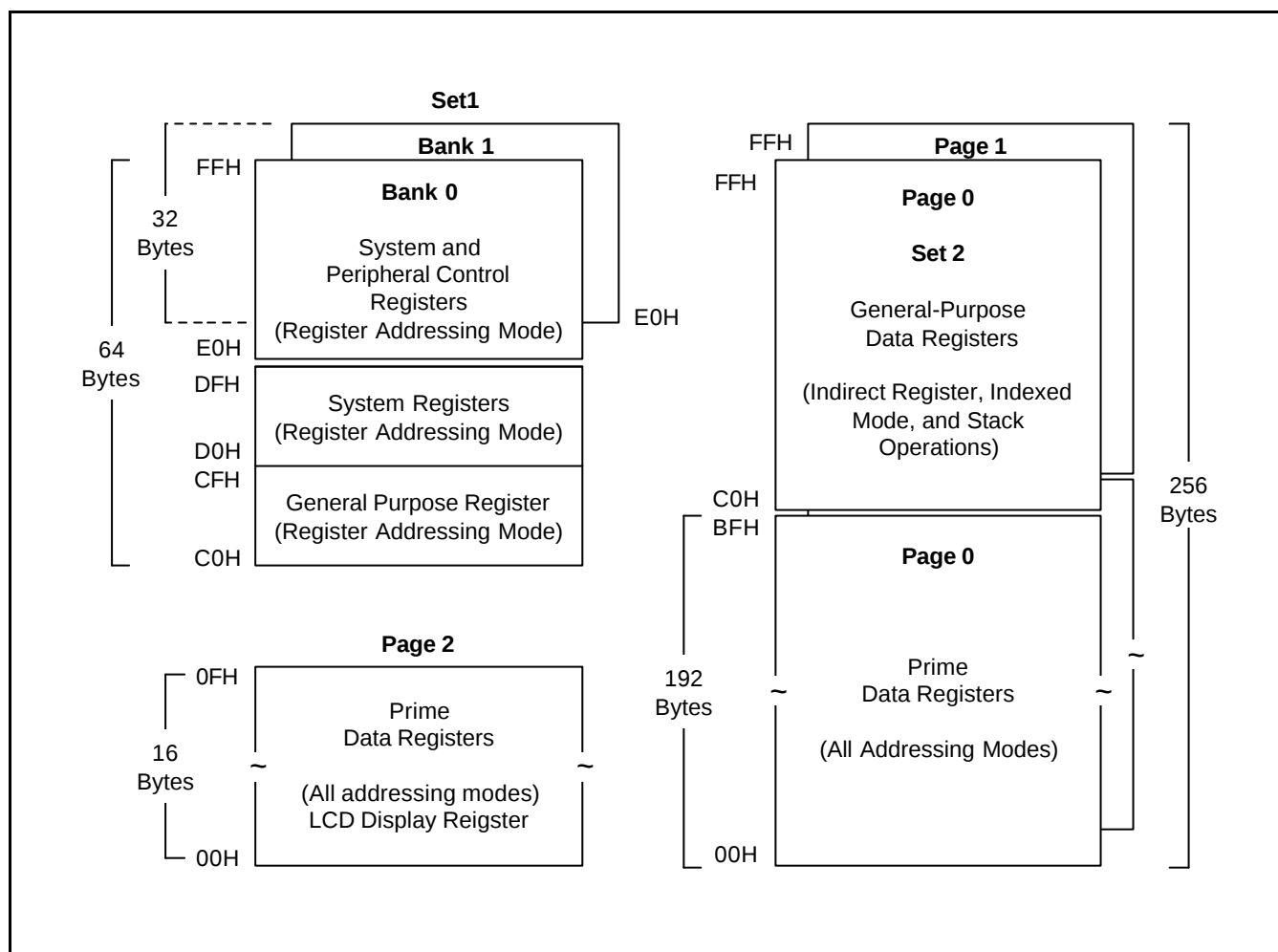
Figure 2-3. Internal Register File Organization (S3C8275)
