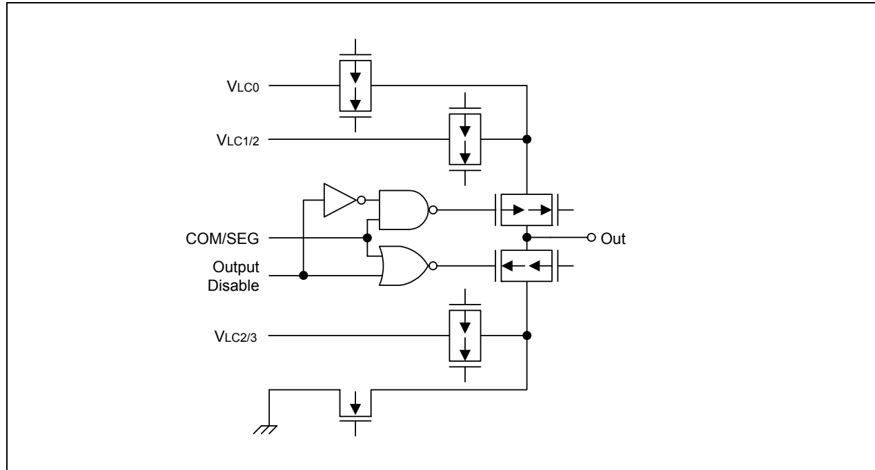
Figure 1-11. Pin Circuit Type H-4
