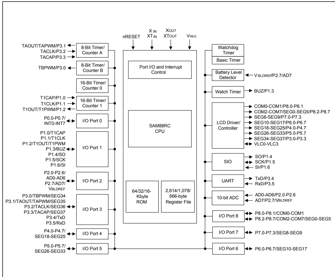
Figure 1-1. Block Diagram
