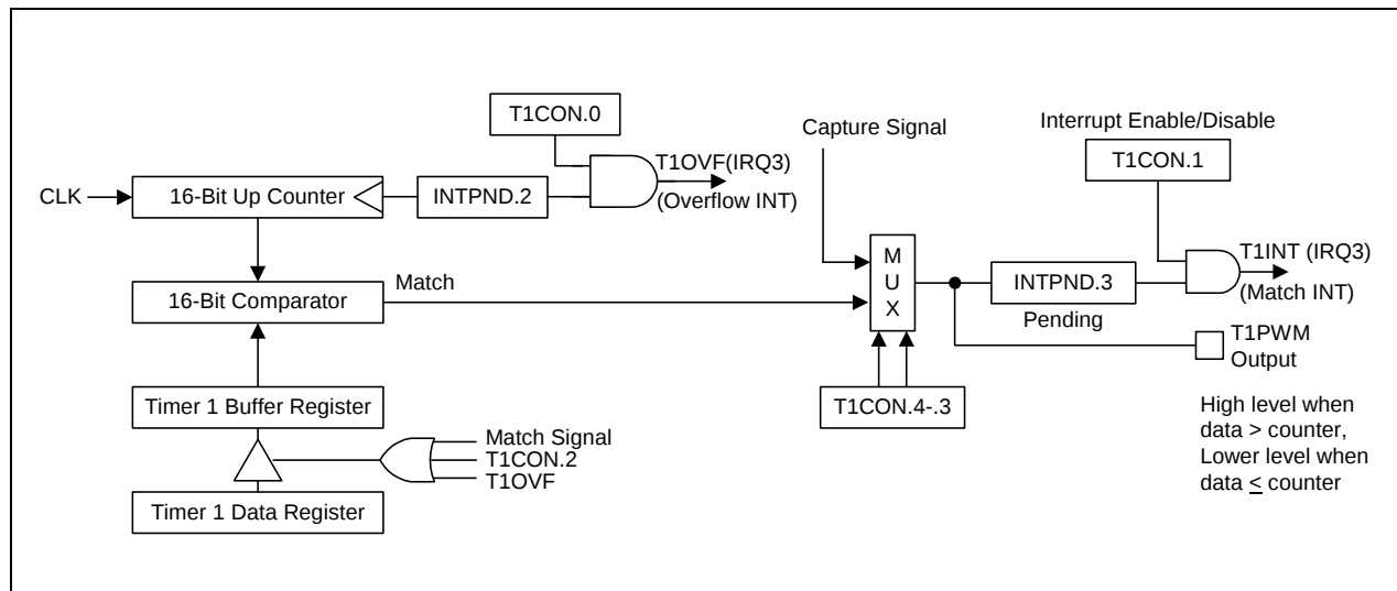
Figure 12-5. Simplified Timer 1 Function Diagram: PWM Mode
