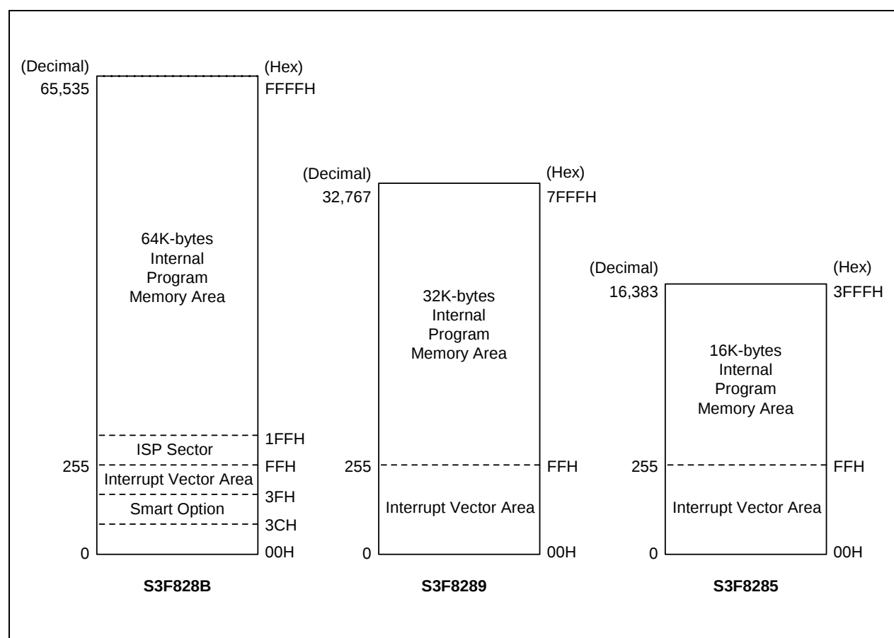
Figure 19-5. Program Memory Address Space
