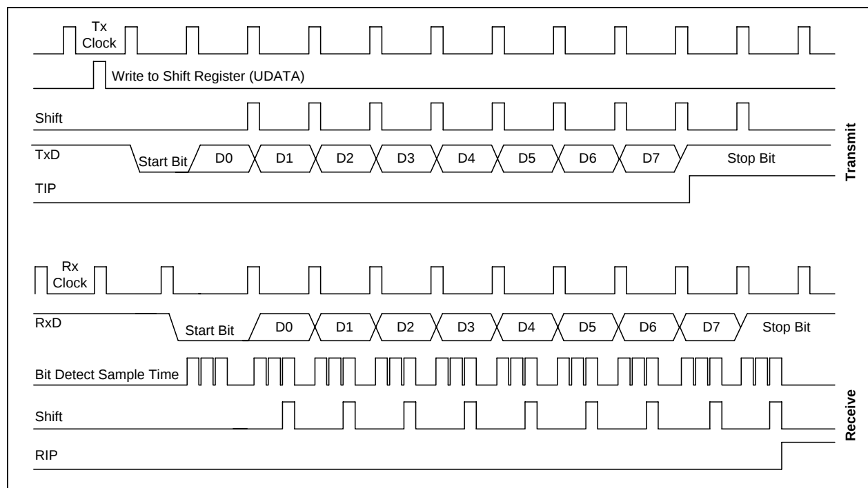
Figure 17-7. Timing Diagram for Serial Port Mode 1 Operation
