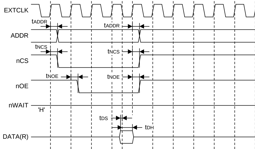
Figure 13-4. SRAM Read Access Timing without nWAIT ( t_{COS}=1, t_{ACS}=0, t_{COH}=0, t_{ACC}=3 )
