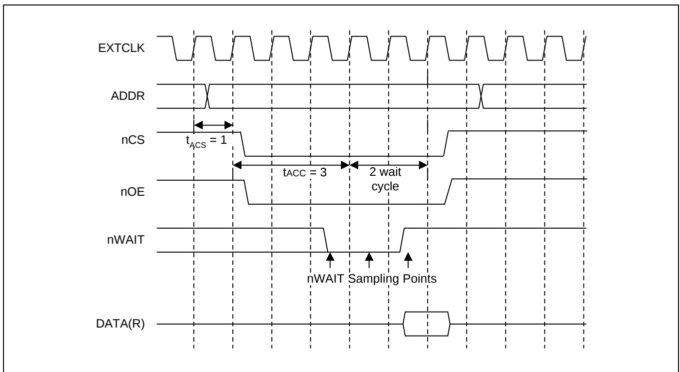
Figure 13-9. SRAM Read Access Timing with nWAIT at the Last Cycle of Half-Word/Word Access and Byte Access (t_{COS}=0, t_{ACS}=1, t_{COH}=0, t_{ACC}=3, \text{external wait}=2)
