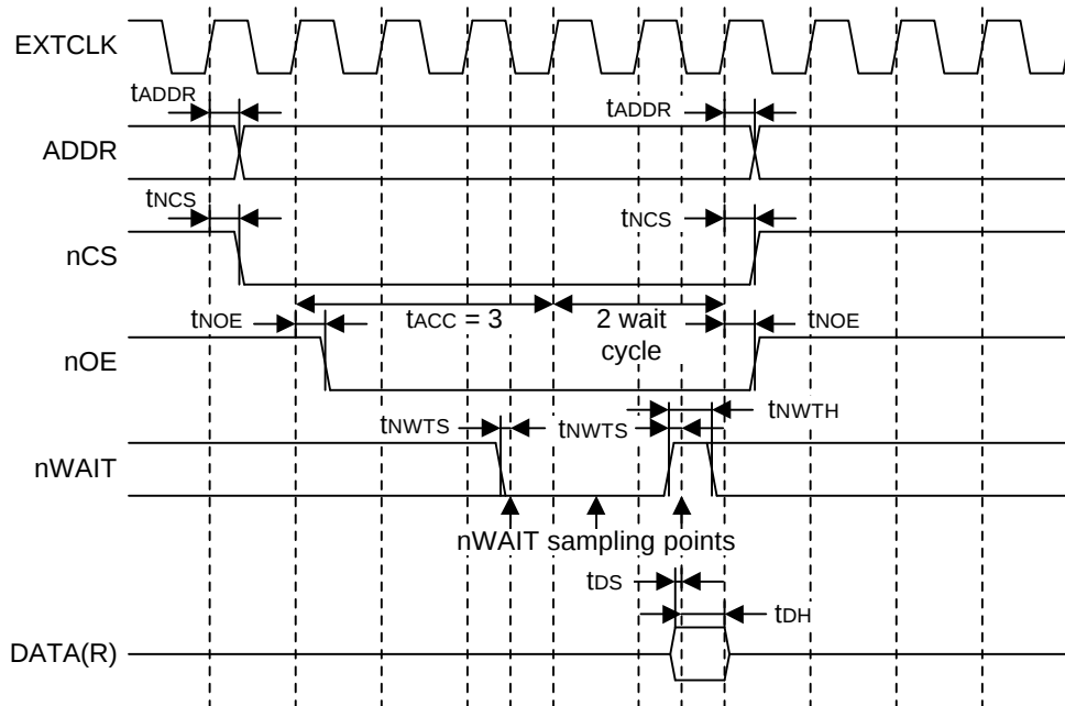
Figure 13-5. SRAM Read Access Timing with nWAIT ( t_{COS}=1, t_{ACS}=0, t_{COH}=0, t_{ACC}=3 , external wait=2 )
