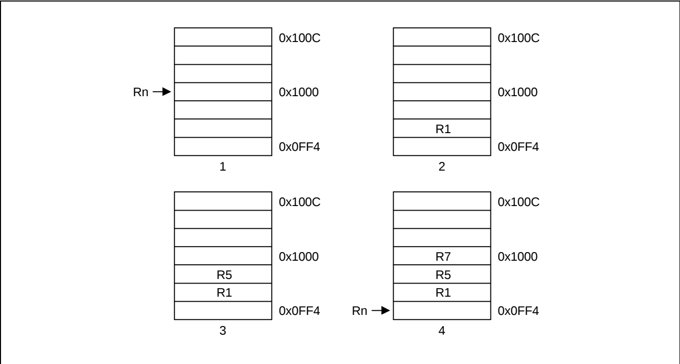
Figure 3-21. Post-Decrement Addressing
