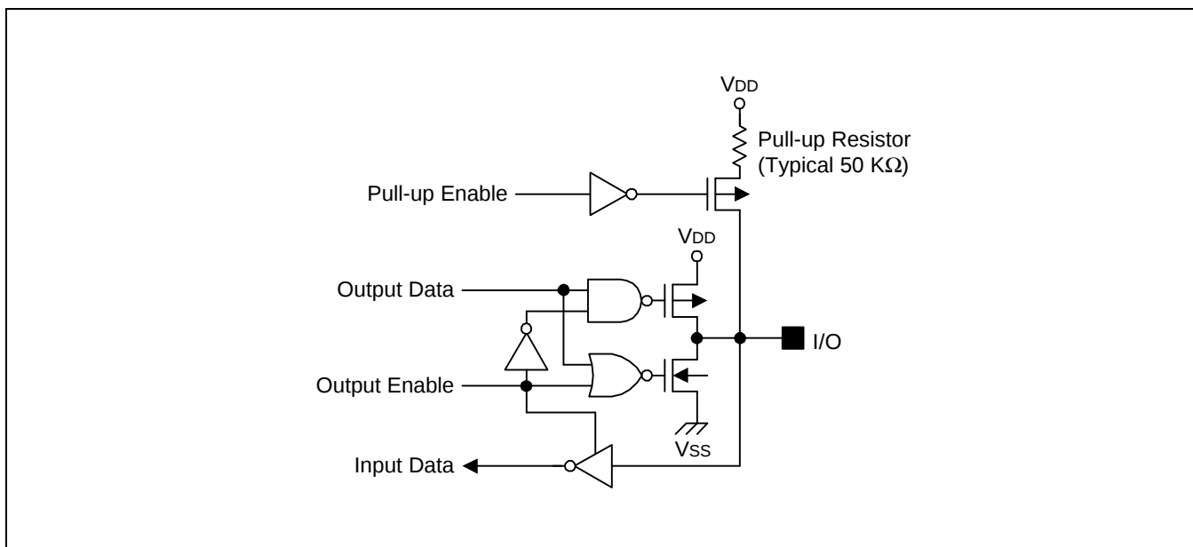
Figure 1-6. IOPU (Input/Output pin with Programmable Pull-up Resistor)
