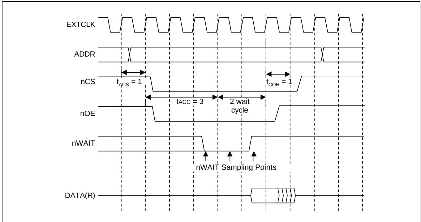
Figure 13-8. SRAM Read Access Timing with nWAIT (t_{COS}=0, t_{ACS}=1, t_{COH}=1, t_{ACC}=3, \text{external wait}=2)
