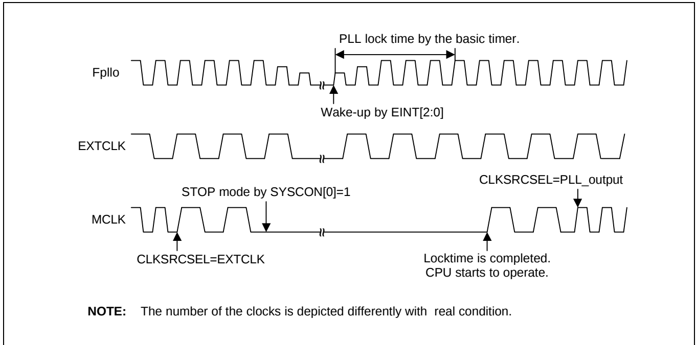
Figure 11-2. Entering &amp; Wake-up in the STOP Mode
