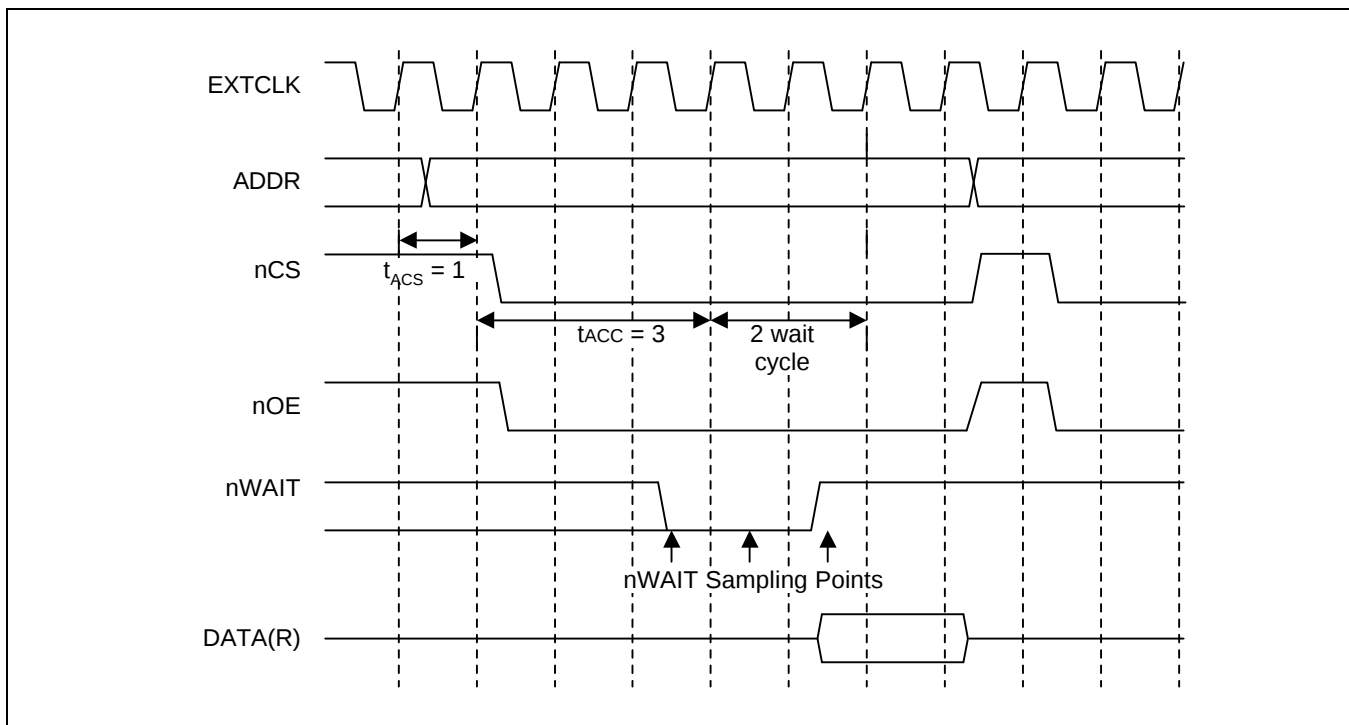
Figure 13-10. SRAM Read Access Timing with nWAIT During Half-Word/Word Access, except the Last Cycle ( t_{\text{COS}}=0 , t_{\text{ACS}}=1 , t_{\text{COH}}=0 , t_{\text{ACC}}=3 , external wait=2)
