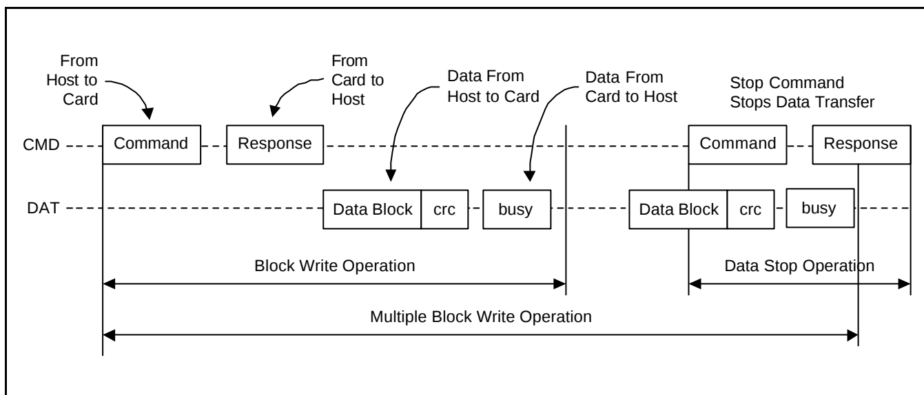
Figure 6. (Multiple) Block Write Operations
