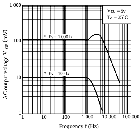
Fig. 10 Frequency Characteristics
