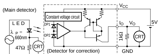
Frequency Characteristics Test Circuit
