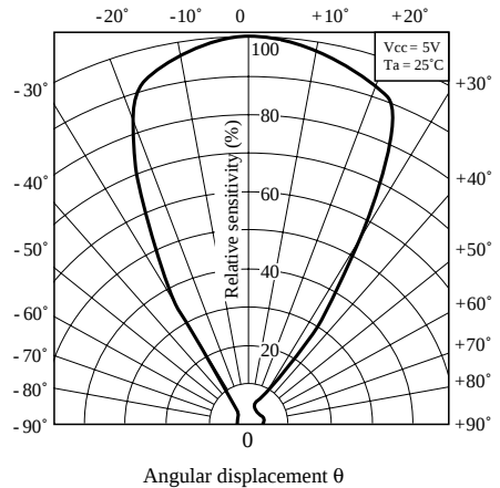
Fig. 12 Radiation Diagram (Top/Bottom Direction)
