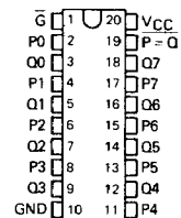
SN54LS688, SN54LS689 ... J PACKAGE SN74LS688, SN74LS689 ... DW, J OR N PACKAGE (TOP VIEW)
