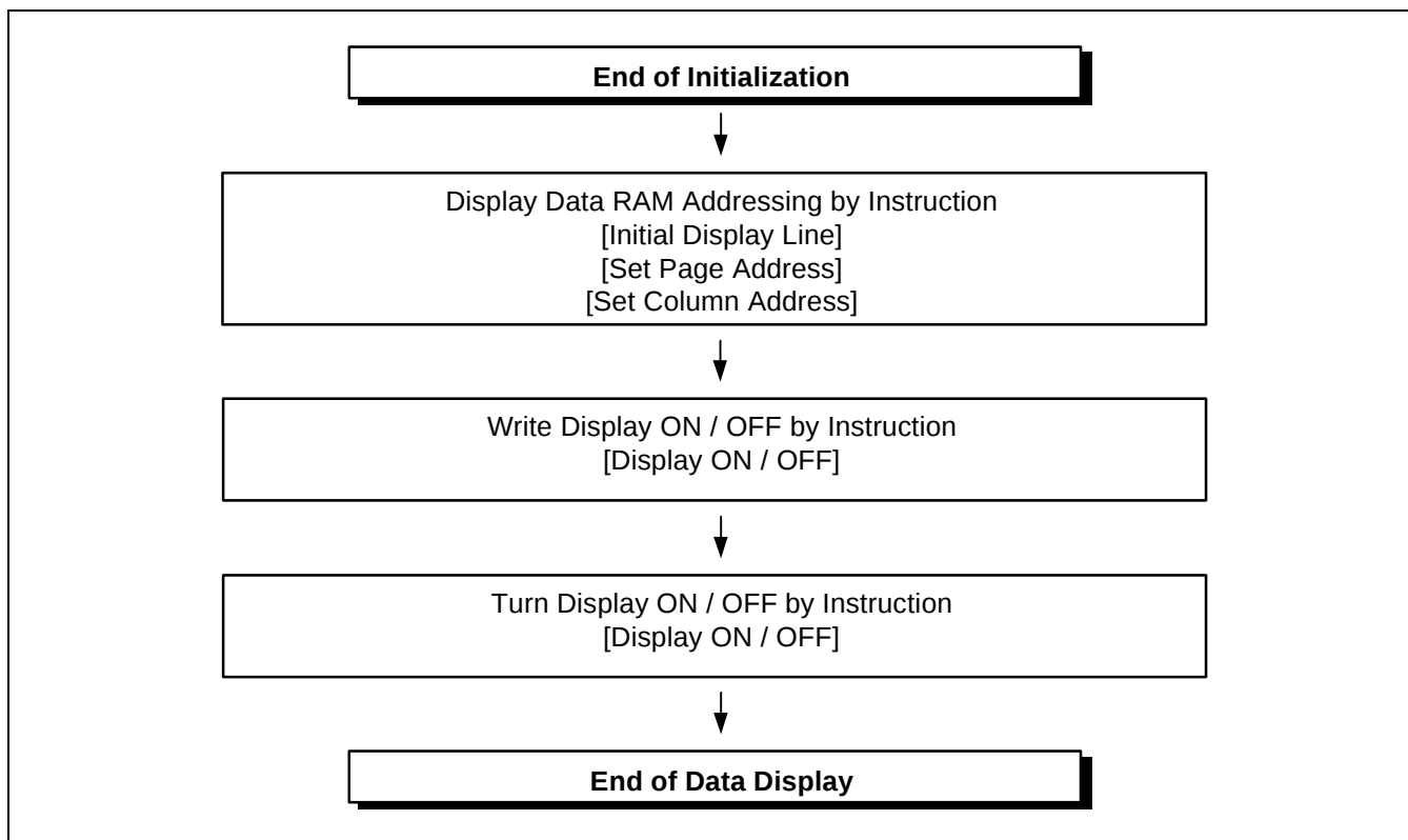
Figure 26. Data Displaying
