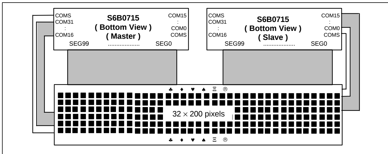
Figure 43. SHL = 0, ADC = 1
