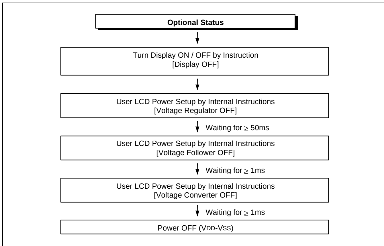
Figure 27. Power OFF
