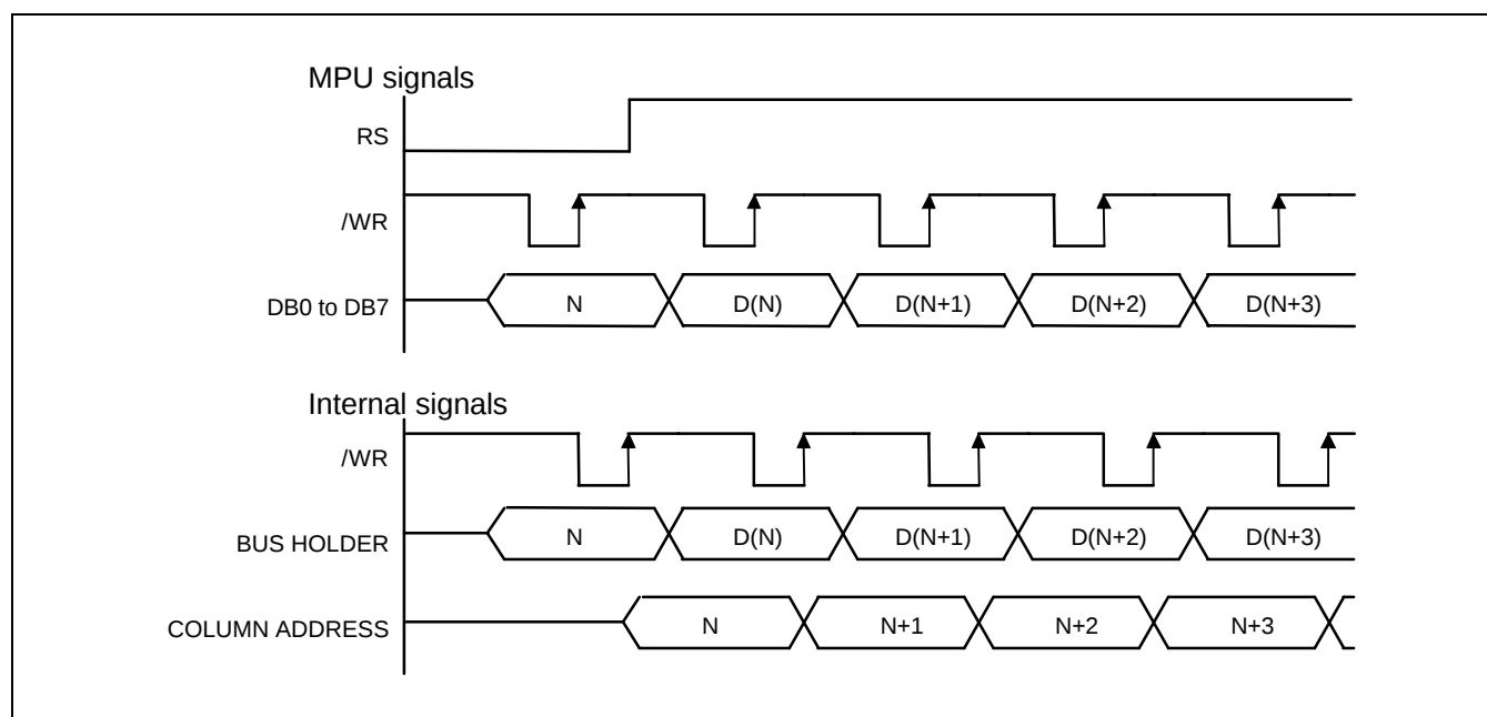
Figure 4. Write Timing
