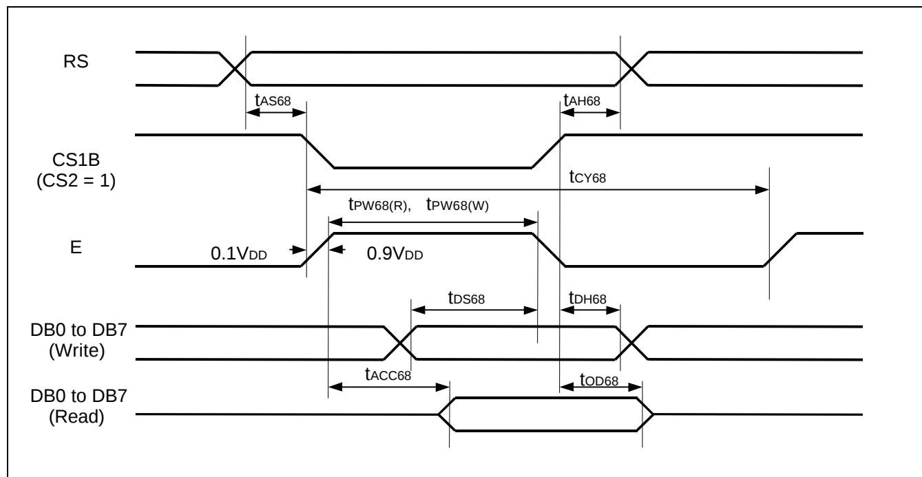
Figure 32. Read / Write Characteristics (6800-series Microprocessor)
