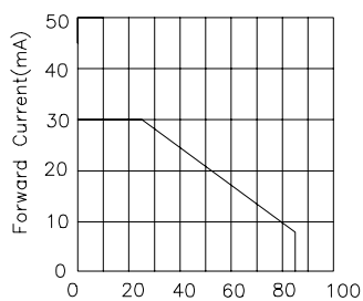
DERATING CURVE
