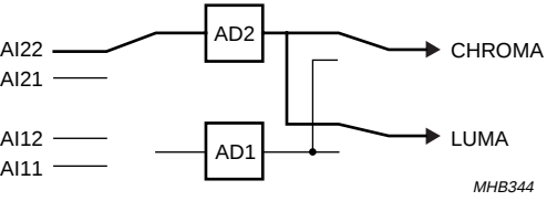
Fig.38 Mode 3; CVBS (automatic gain).
