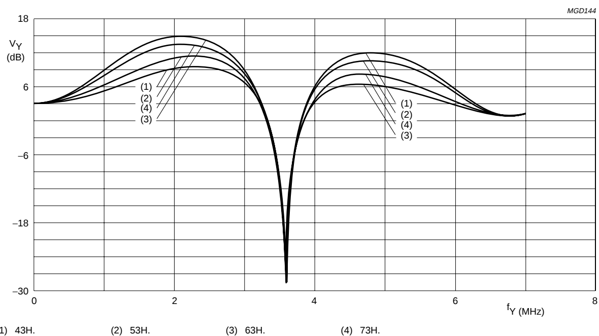
Fig.16 Luminance control SA 09H, 3.58 MHz trap/CVBS mode, prefilter on, different aperture band-pass centre frequencies.
