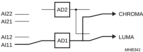
Fig.35 Mode 0; CVBS (automatic gain).
