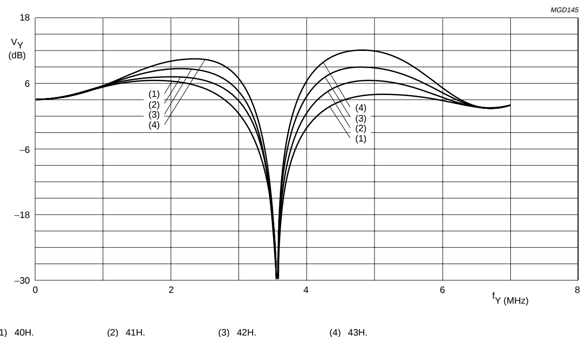
Fig.17 Luminance control SA 09H, 3.58 MHz trap/CVBS mode, prefilter on, different aperture factors.
