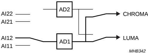
Fig.36 Mode 1; CVBS (automatic gain).
