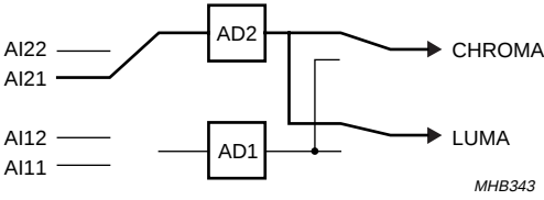
Fig.37 Mode 2; CVBS (automatic gain).
