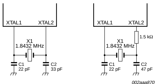
Fig 7. Crystal oscillator connection
