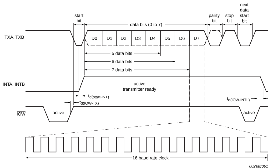
Fig 17. Transmit timing
