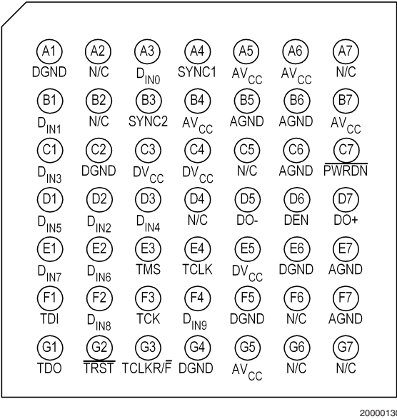
SCAN921023SLC - Serializer (Top View)
