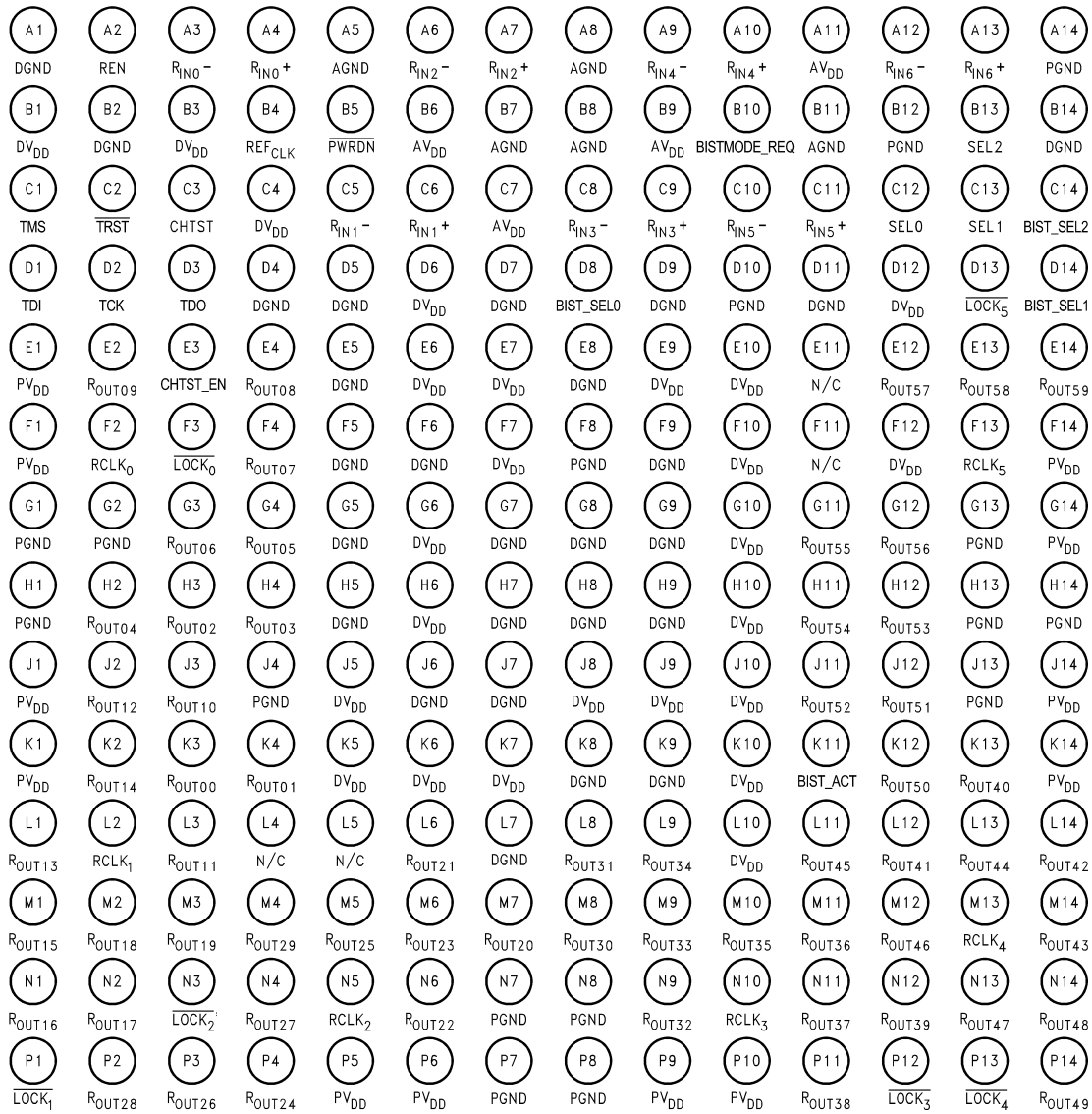
SCAN921260UJB and SCAN921260UJBX (196 pin LPGA)
