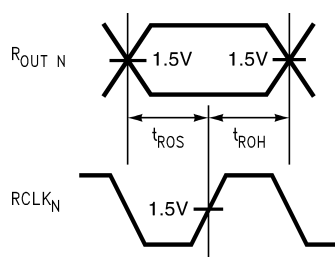
FIGURE 2. Output Timing t_{ROS} and t_{ROH}
