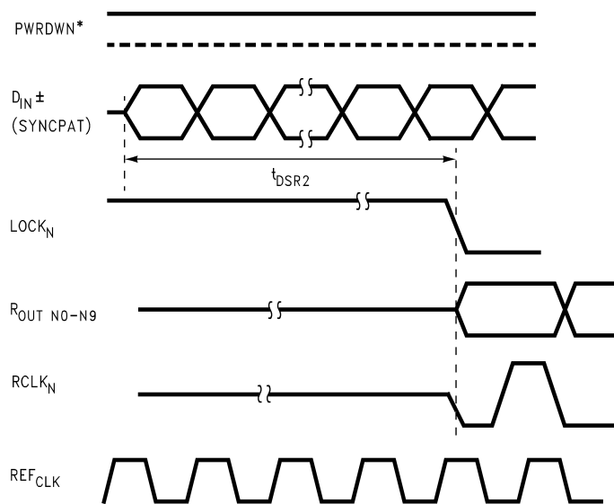
FIGURE 4. Locktime to SYNCPAT t_{DSR2}
