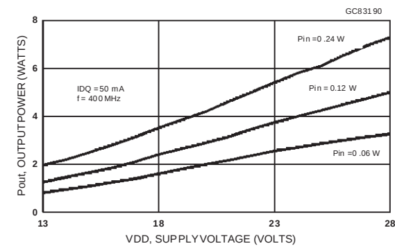
Output Power vs Voltage Supply
