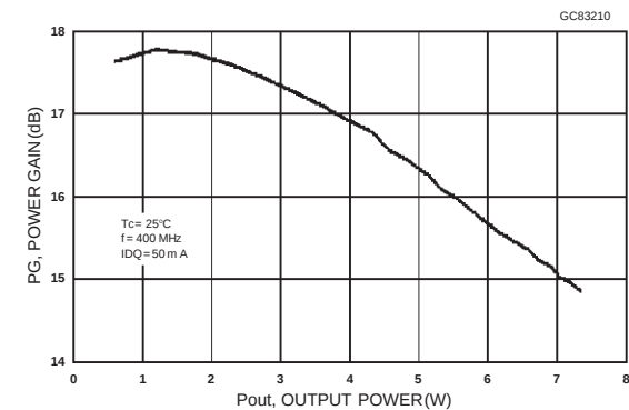
Power Gain vs Output Power
