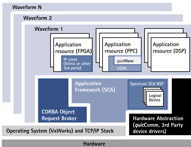
Figure 2. SDR-3000 Software Stack
