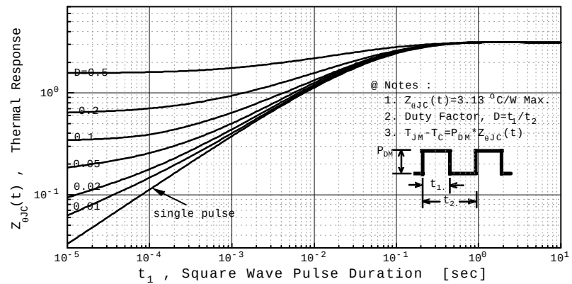
Fig 11. Thermal Response
