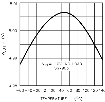
FIGURE 3. TEMPERATURE COEFFICIENT
