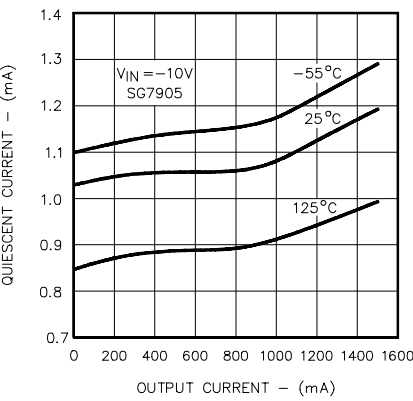
FIGURE 2. QUIESCENT CURRENT VS. LOAD
