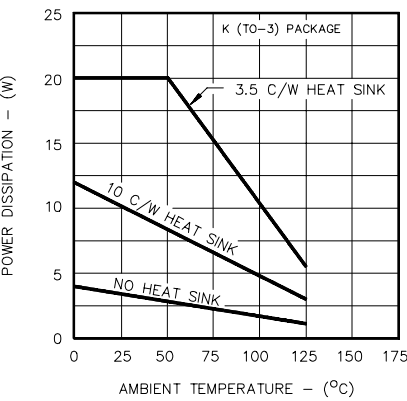
FIGURE 1. MAXIMUM AVERAGE POWER DISSIPATION
