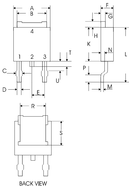
TO-252AA (DPak)
