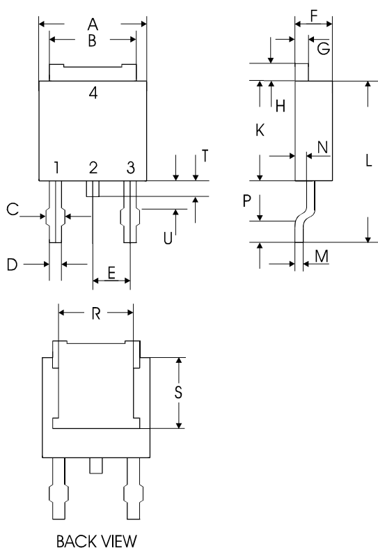
P-TO252 (D-Pak)
