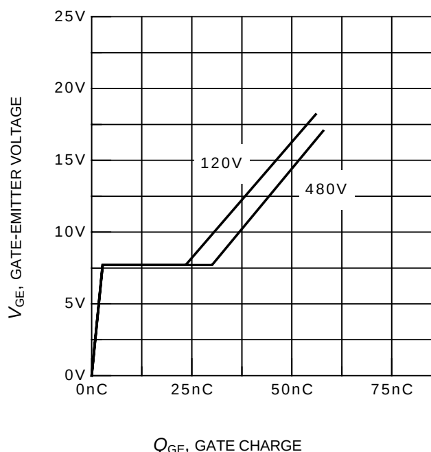
Figure 17. Typical gate charge ( I_C = 10A )
