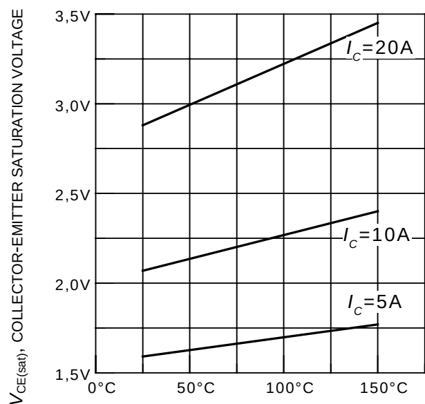
Figure 8. Typical collector-emitter saturation voltage as a function of junction temperature ( V_{GE} = 15V )
