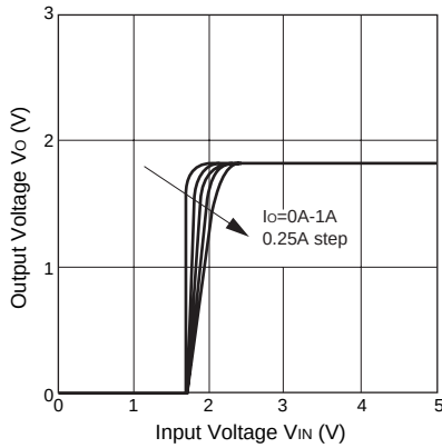
Line Regulation
