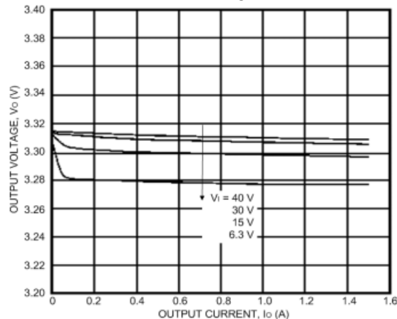
■ Load Regulation
