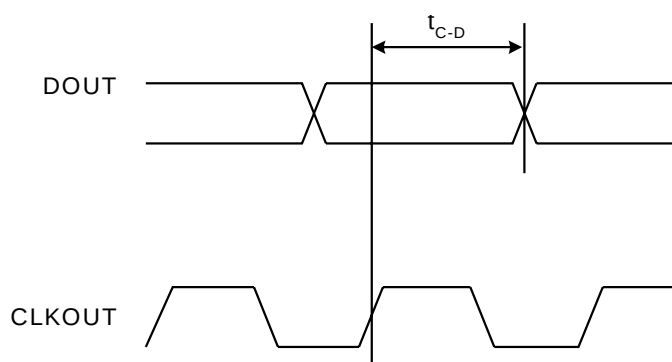
Figure 3. Clock to Data Timing
