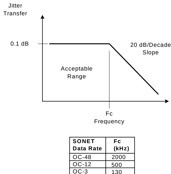
Figure 9. Jitter Transfer Specification
