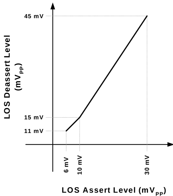
Figure 7. Hysteresis Dependency
