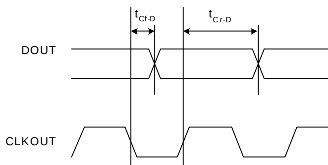
Figure 3. Clock to Data Timing
