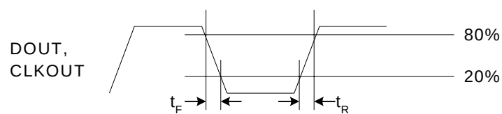
Figure 4. DOUT and CLKOUT Rise/Fall Times
