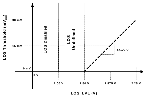
Figure 6. LOS_LVL Mapping
