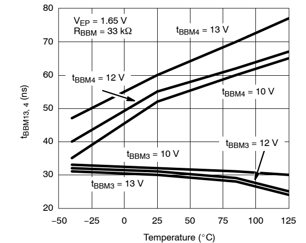
t_{BBM3, 4} vs. Temperature, V_{EP} = 1.65 V
