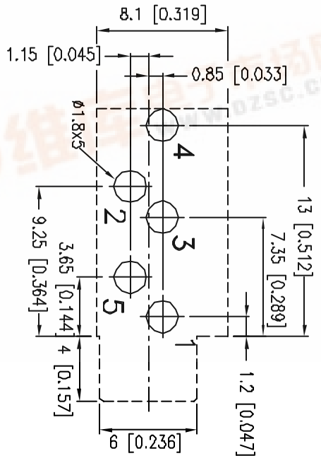
HOLE LAYOUT (TOP VIEW)
