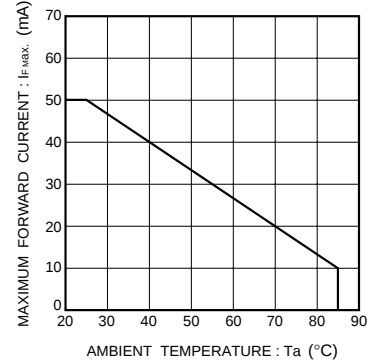
Fig.10 Maximum forward current vs. ambient temperature (Derating)
