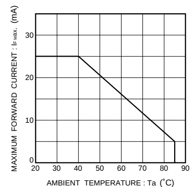
Fig.16 Maximum forward current vs. ambient temperature (Derating)
