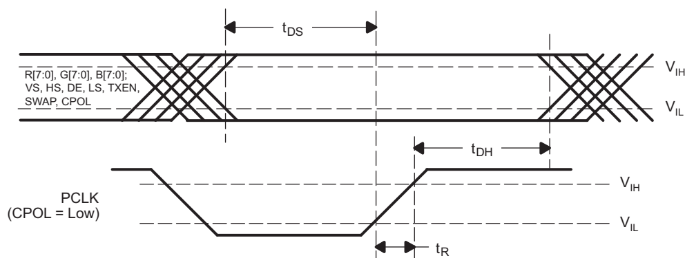
Figure 6. Setup/Hold Time
