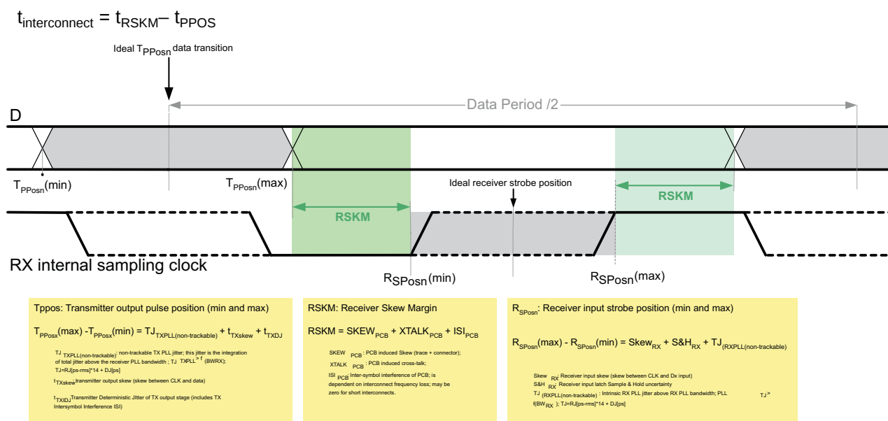
Figure 30. Jitter Budget
