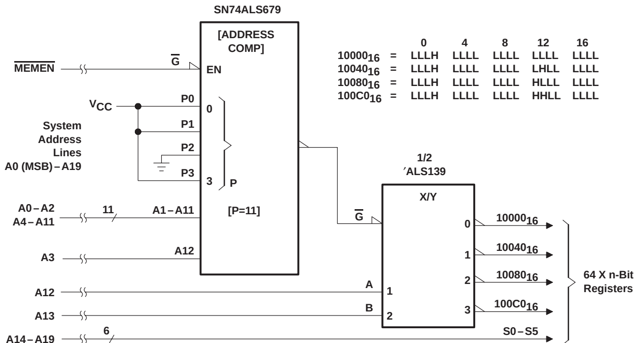
Figure 1. Register-Bank Decoder
