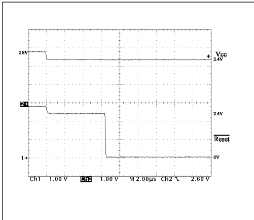
Figure 7A. SP706 \overline{RESET} Response Time
