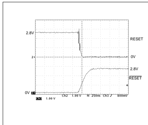
Figure 9. SP708 \overline{RESET} and \overline{RESET} De-Assertion
