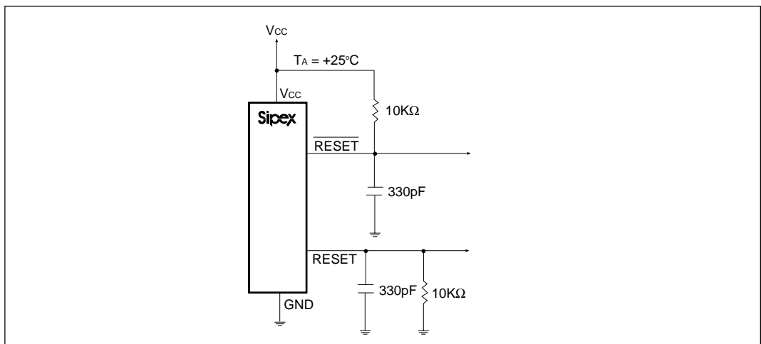
Figure 10. Circuit for the SP708 \overline{RESET} and \overline{RESET} Assertion and De-Assertion
