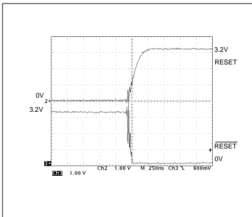
Figure 8. SP708 \overline{RESET} and \overline{RESET} Assertion
