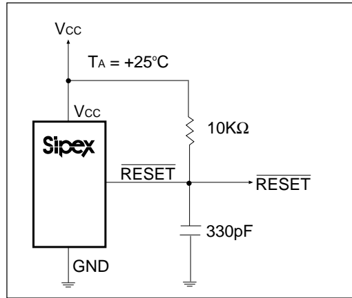
Figure 7B. Circuit for the SP706 \overline{RESET} Response Time
