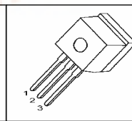
P-TO262-3-1
